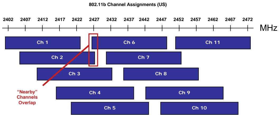
Figure 2. 802.11b Channel Assignments
