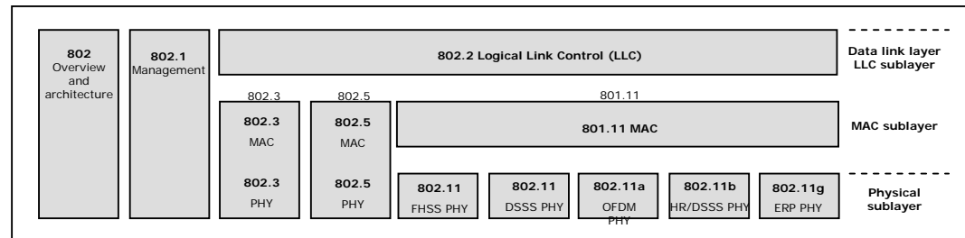
Figure 1. 802.11 data link and physical layers
