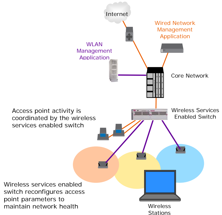
Figure 4. A centrally controlled wireless network
