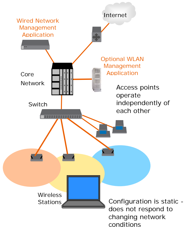
Figure 3. Wireless network consisting of standalone access points
